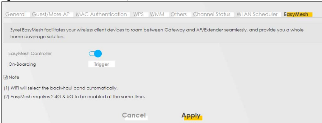
Figure 100 Network > Wireless > EasyMesh
