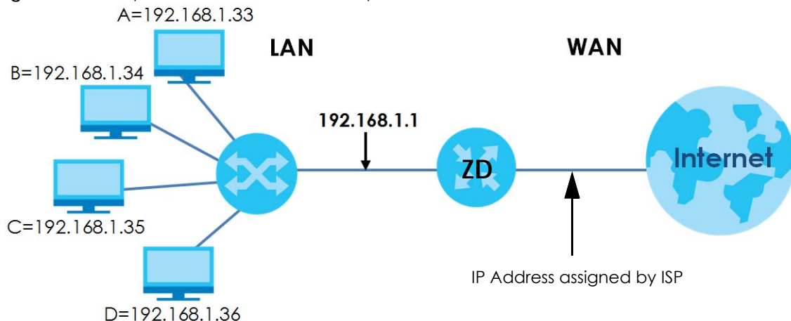
Figure 142 Multiple Servers Behind NAT Example
