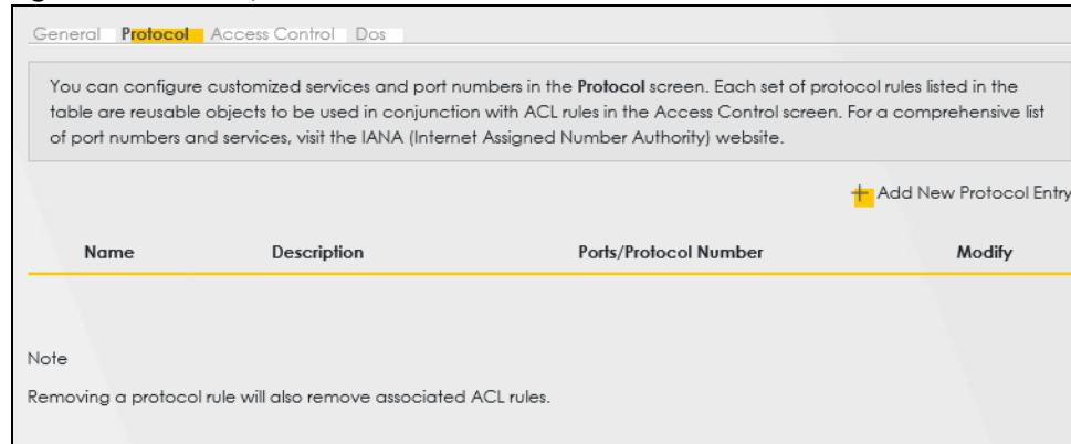
Figure 151 Security > Firewall > Protocol
