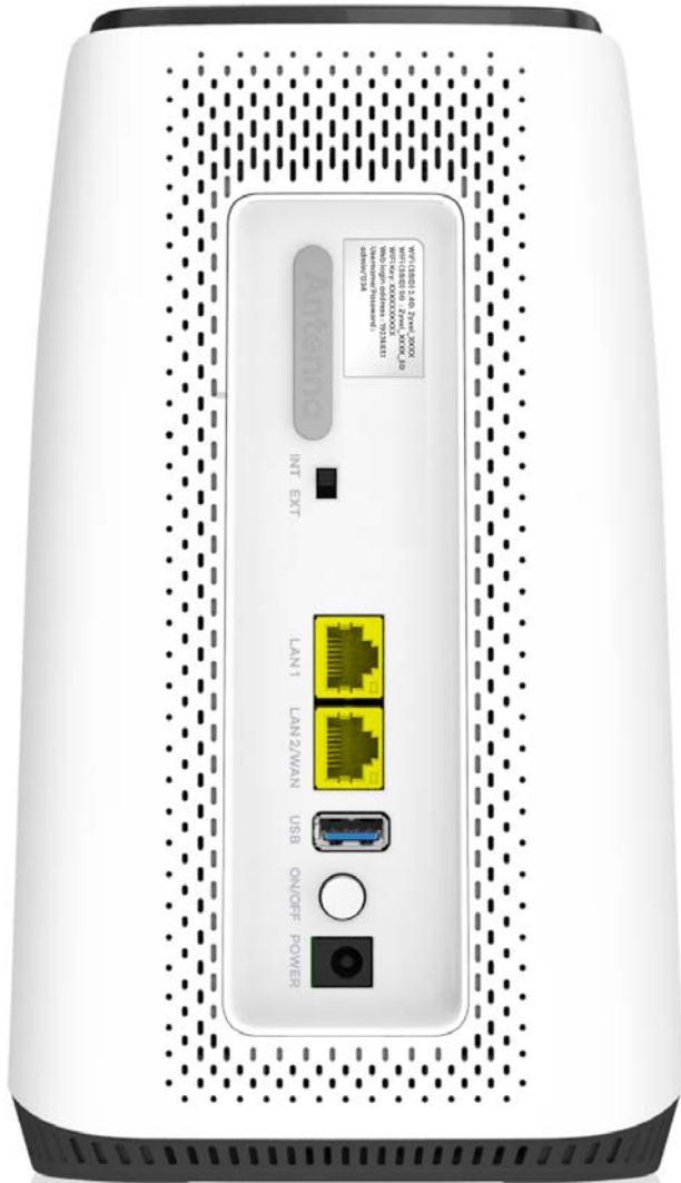
Figure 28 NR5103 / NR5103E / FWA510 Ports and Buttons
