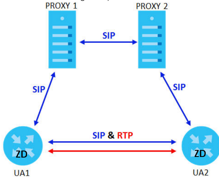
Figure 184 SIP Call Through Proxy Servers
